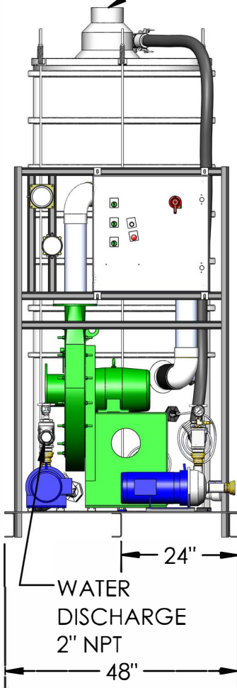
FRONT VIEW
